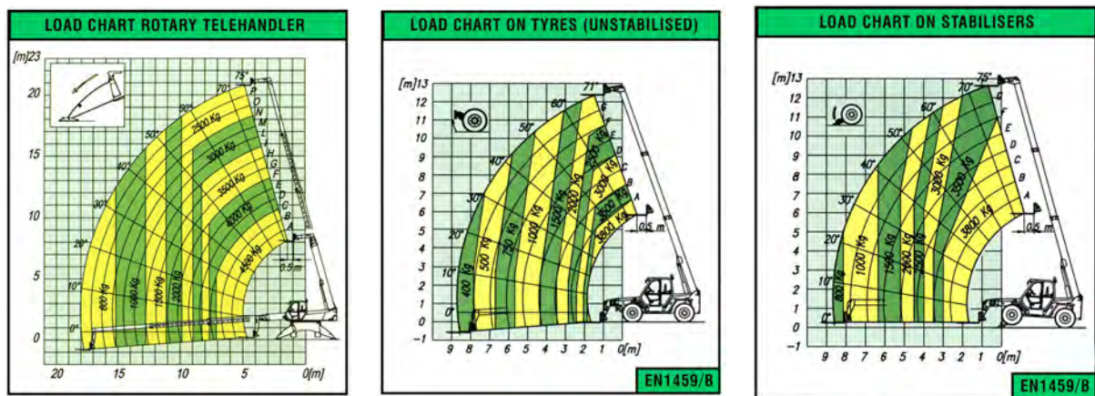
Figure 12 – Typical Load Charts
