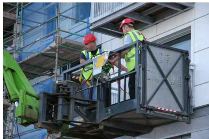
Figure 20 - Integrated Work Platform
